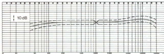
Standard response curve with tolerances
