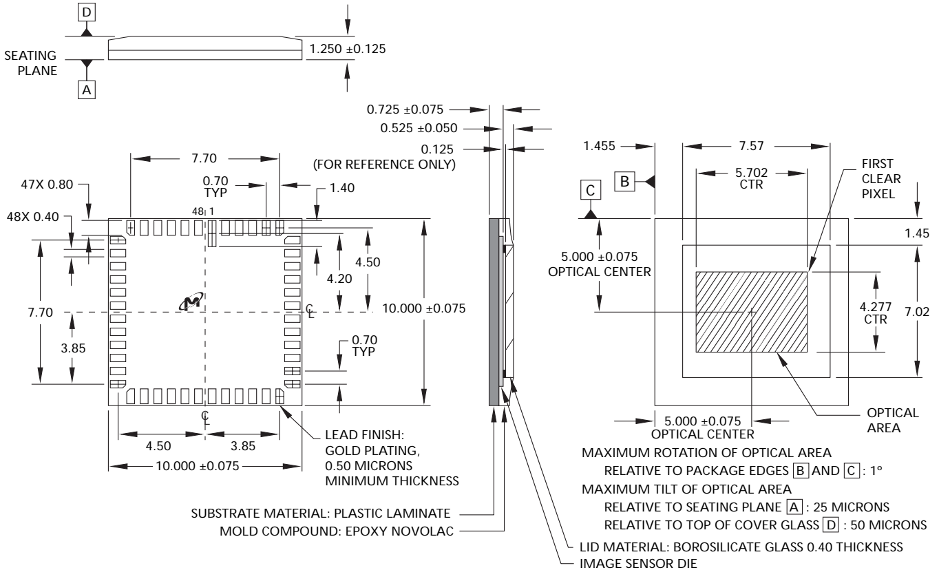
Figure 30: 48-Pin iLCC Package Outline
