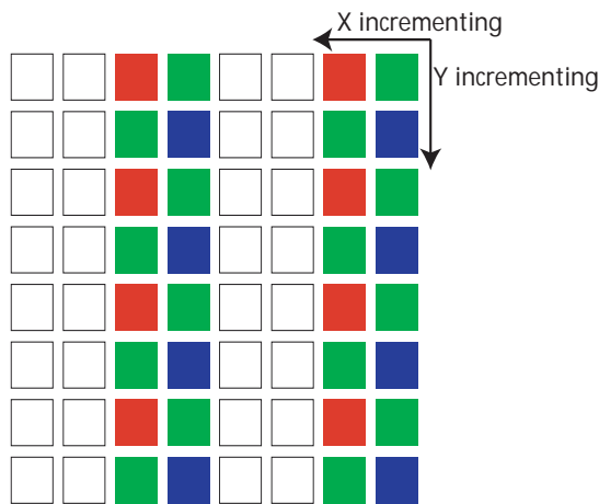
Figure 16: Pixel Readout (Column Skip 2X)
