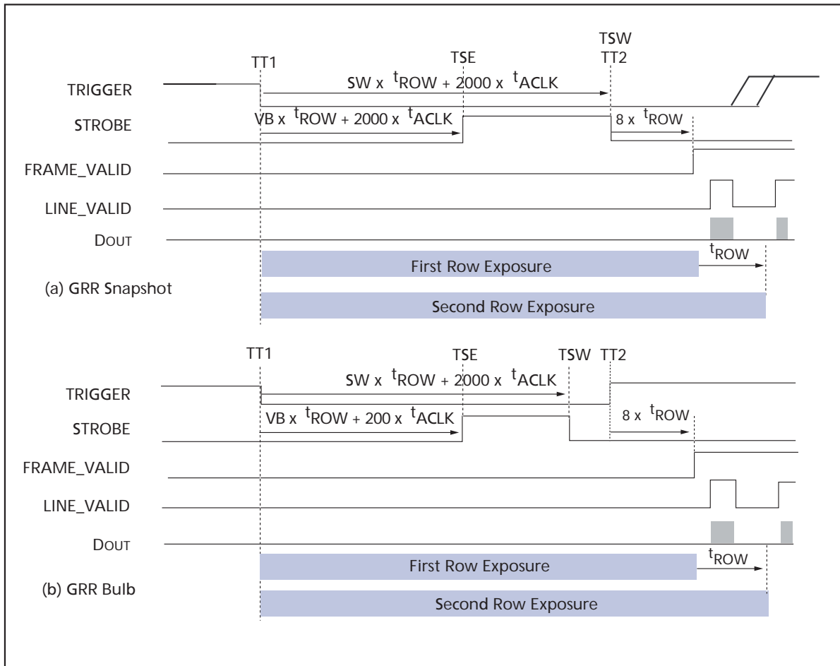
Figure 24: GRR Snapshot Timing
