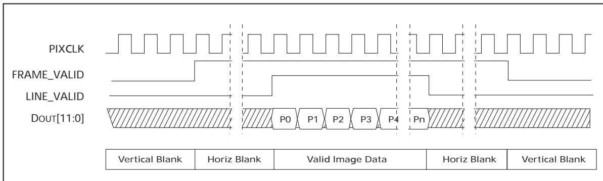
Figure 8: Default Pixel Output Timing
