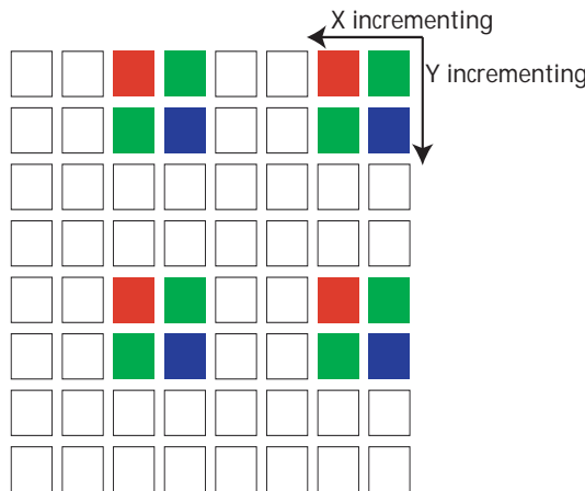
Figure 18: Pixel Readout (Column Skip 2X, Row Skip 2X)
