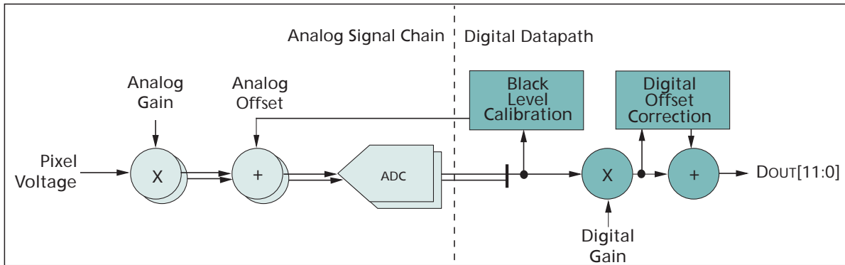
Figure 25: Signal Path
