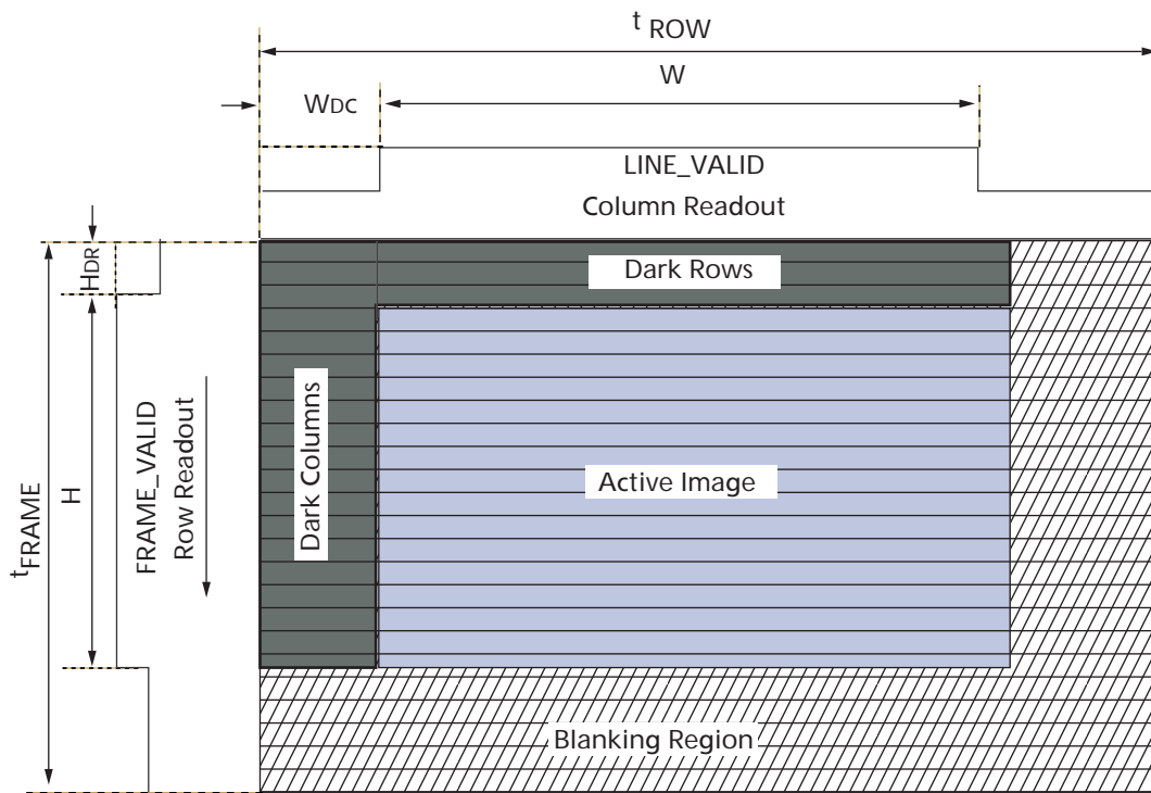
Figure 10: Frame Timing
