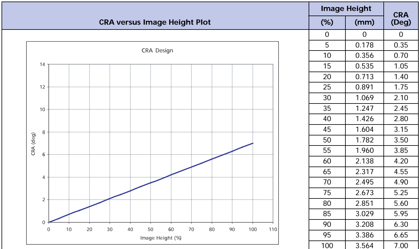
Figure 27: CRA versus Image Height
