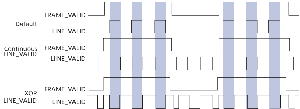
Figure 9: LINE_VALID Format Options
