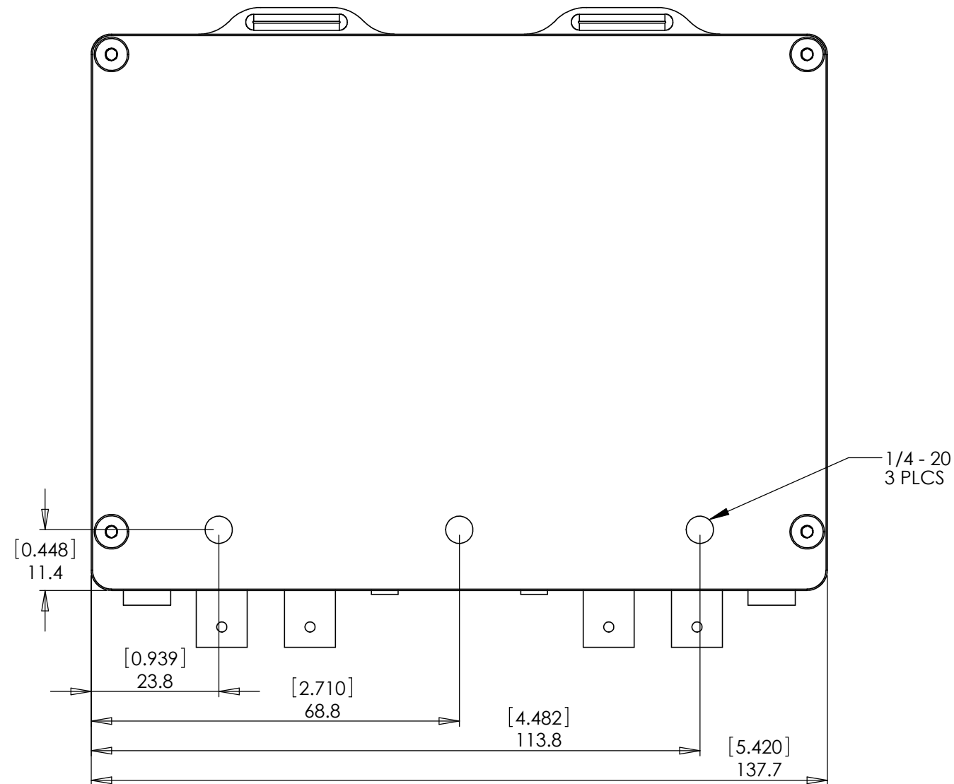
REAR
